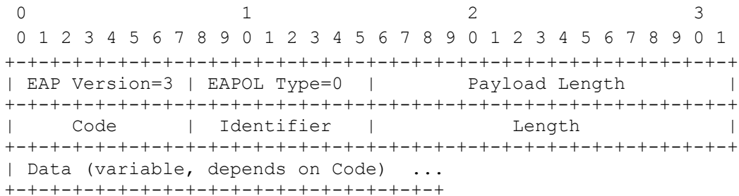
Figure 21: Packet Payload for EAPOL Type=0
