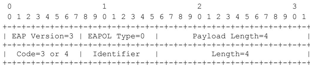
Figure 33: Packet Payload Format for Success/Failure Packets
